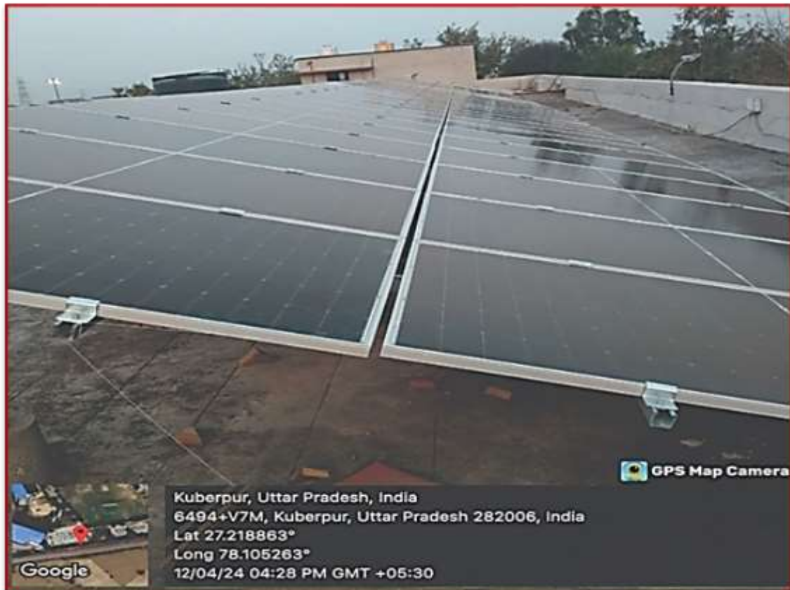
Solar Power System University Campus – 70KWh
